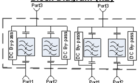
Block Diagram (x2)
