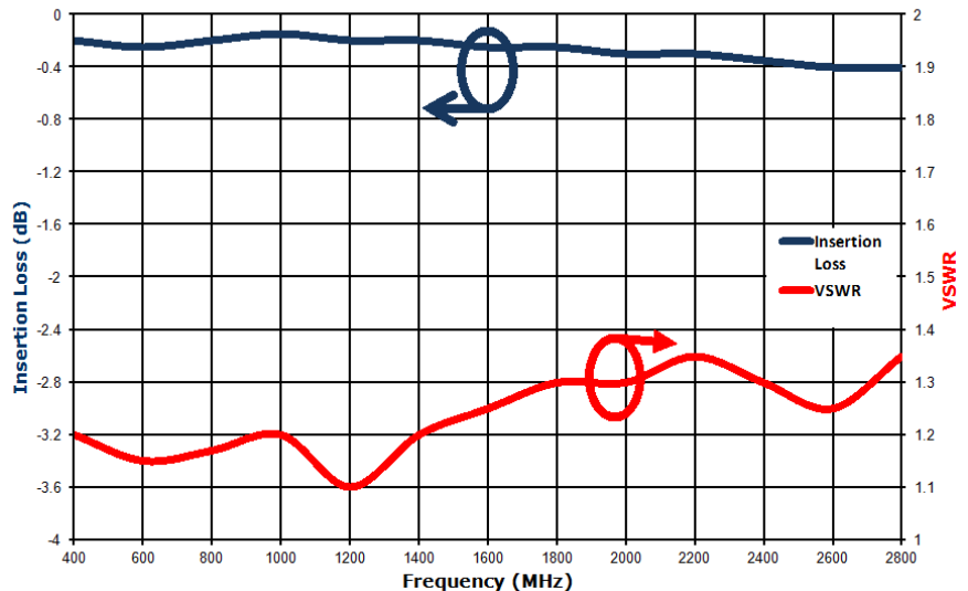
Insertion Loss & VSWR
