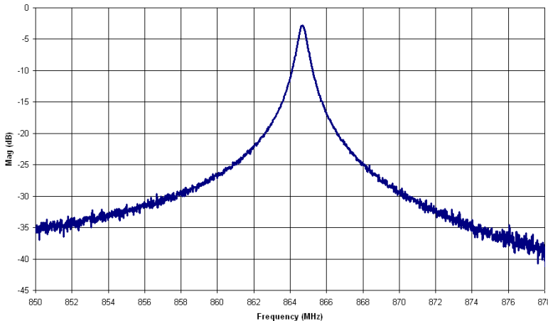
Typical Response of a Single Cavity Filter Tuned for Insertion Loss of 2.5 dB
